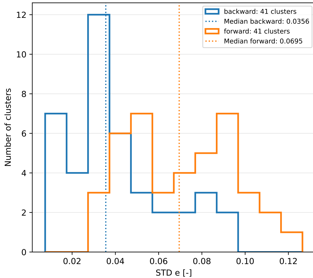
K=41 | Within-cluster STD distributions | Each cluster counts once
